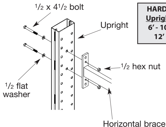
DIAGRAM C BRACE CONNECTION FOR END UPRIGHTS
