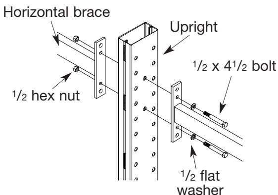
DIAGRAM D BRACE CONNECTION FOR INTERIOR UPRIGHTS
